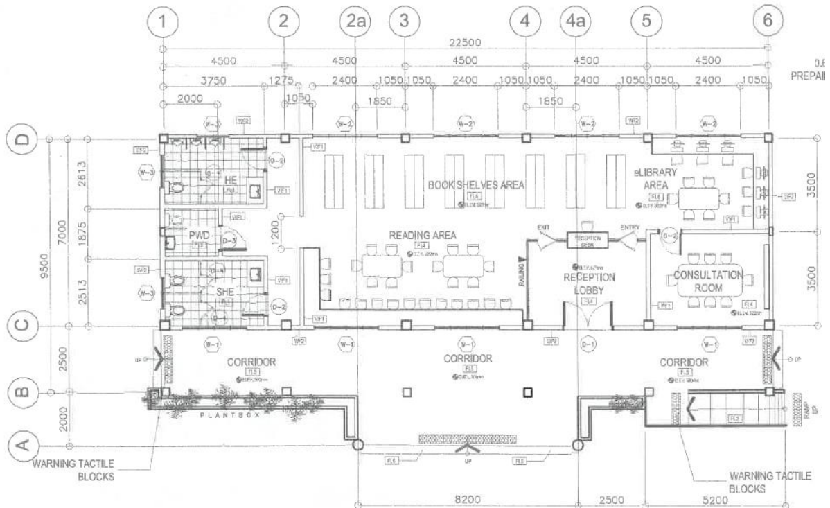
1 GROUND FLOOR PLAN A-2 SCALE 1:100M
