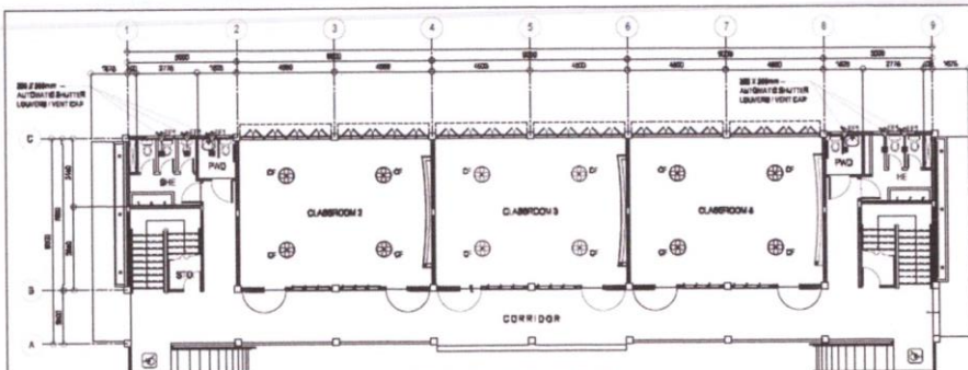
VENTILATION & CEILING FAN LAYOUT GROUND FLOOR PLAN M 3-1 SCALE
