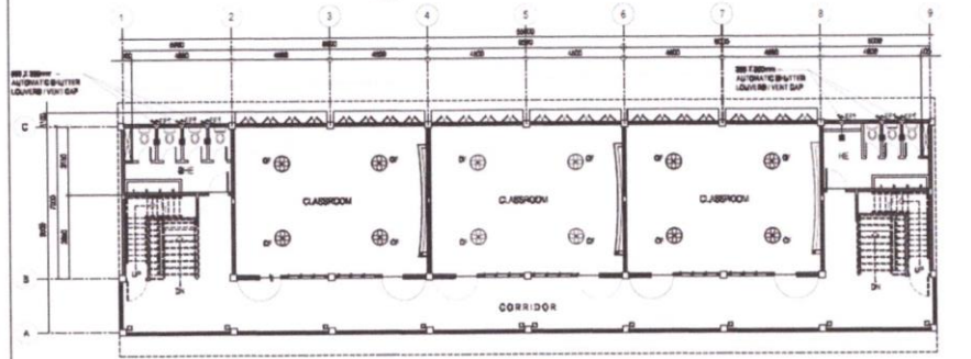
VENTILATION & CEILING FAN LAYOUT SECOND FLOOR PLAN M 3-2 SCALE
