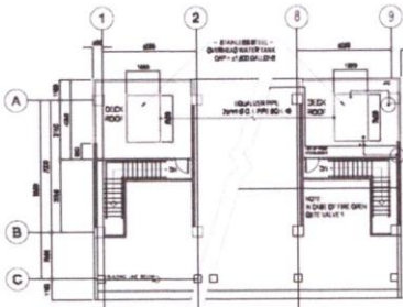
(SHOWING OVERHEAD WATER TANK) PARTIAL ROOF DECK PLAN WP 4-2 SCALE
