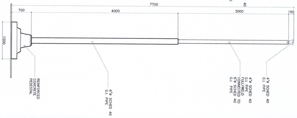
PEDESTAL ELEVATION DETAIL
